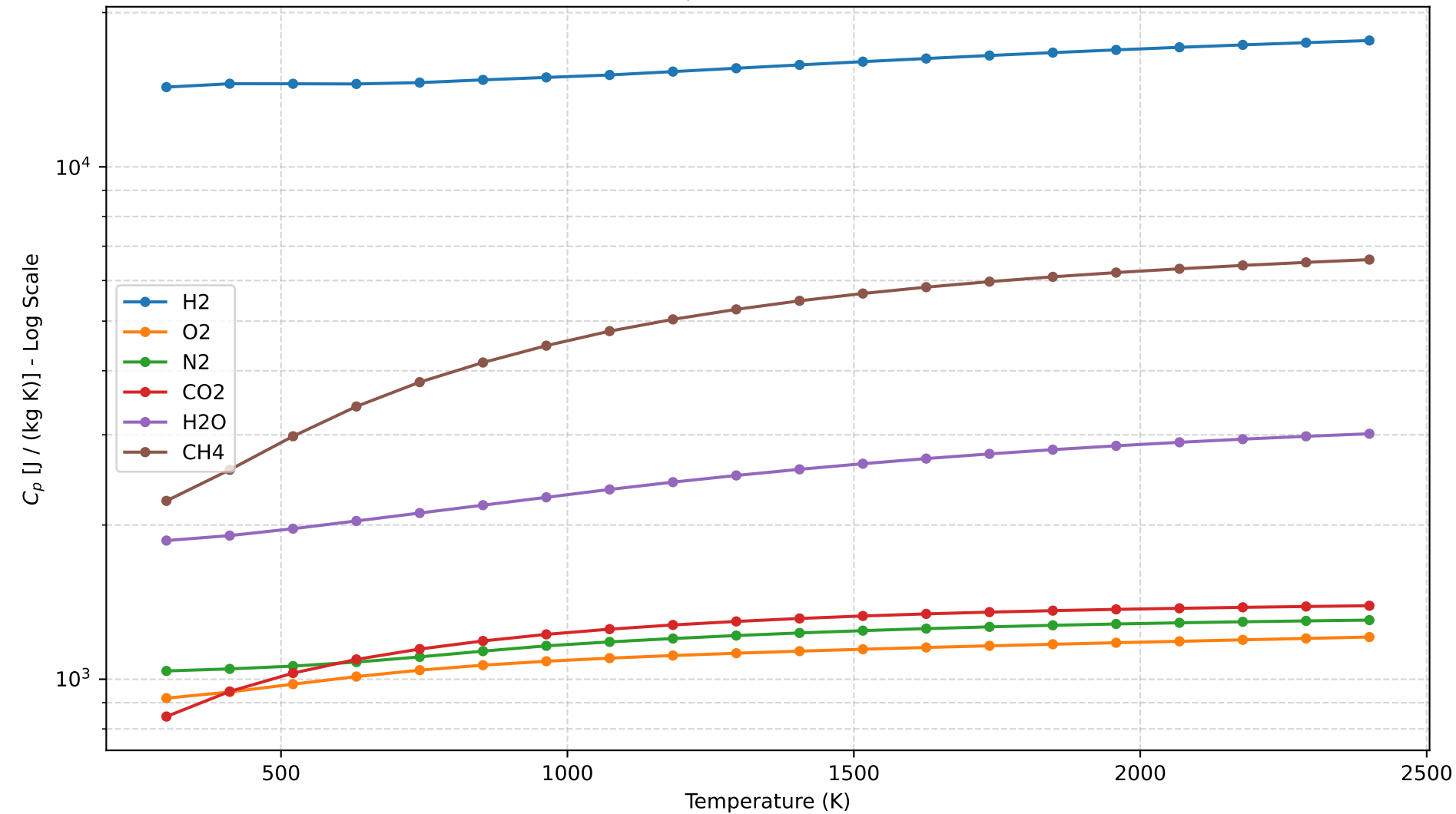
Variation of Specific Heat ( C_p ) with Temperature Using using Cantera
